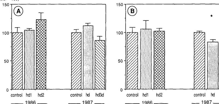
Fig. 4. Normalized estimated parameter values of the initial light use efficiency \epsilon of flag leaves of winter wheat treated with honeydew substitute. A: one day (hd1, hd2, hd3d); B: fifteen days after treatment.
