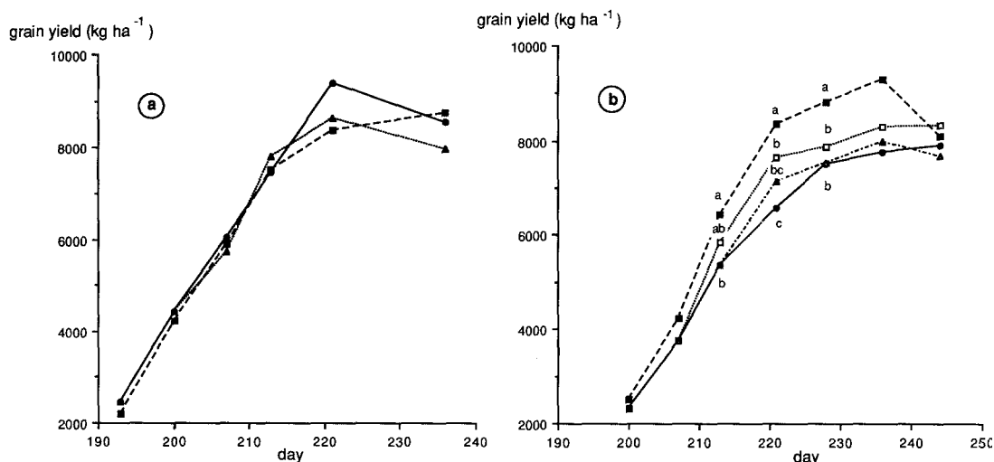
Fig. 6. Grain yield (kg ha -1 ) at 'de Bouwing' (a) and 'de Eest' (b). Treatments at 'de Bouwing' are A (-----■-----), B (.....▲.....) and E (—●—). No significant differences between treatments were found. Treatments at 'de Eest' are A (-----■-----), C (.....□.....), D (.....▲.....) and E (—●—). Similar or no letters for a treatment indicate no significant differences ( p < 0.05 ). A description of the treatments is given in the text.
